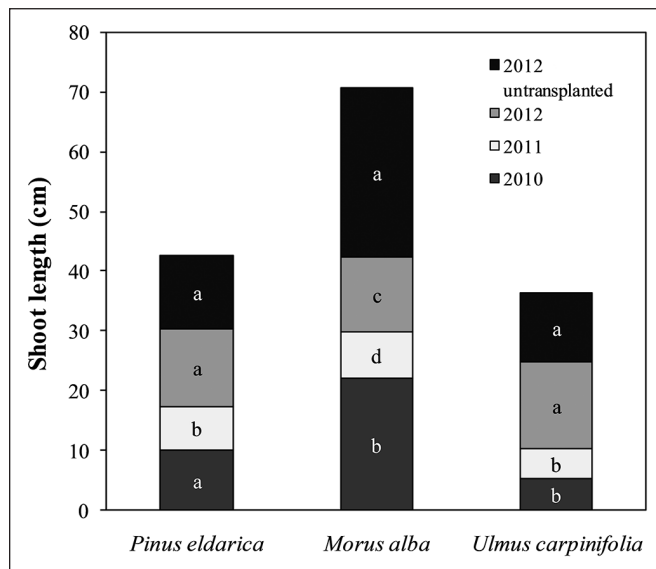
Figure 2. Annual shoot growth of transplanted eldarica pine ( Pinus eldarica ), white mulberry ( Morus alba ), and smoothleaf elm ( Ulmus carpiniifolia ) trees during three years following transplanting. Means followed by the same letter are not significantly different (Duncan's multiple-range test) at 5% level.
