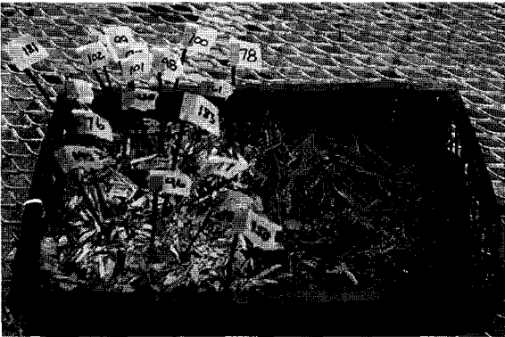
Figure 1. Germination of Thuja occidentalis seeds on a soil monolith from the non-regenerating area of the Enchanted Forest of Fort Témiscamingue. Germinating seedlings are marked with a flag. The left section of the monolith was treated with a 3 cm layer of wood chips whereas the right section of the monolith was untreated. Both sections were seeded with 100 T.occidentalis seeds.
