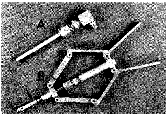
Figure 1. Standard tip with tapered shaft for angled injection (A) and tip created for straight-in injection (B). Expandable rubber tubing which creates the seal in the straight hole indicated by arrow.
