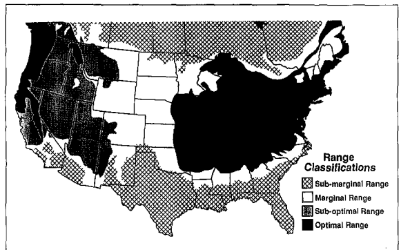
Figure 2. North American climatic range classifications of Acer platanoides L.
