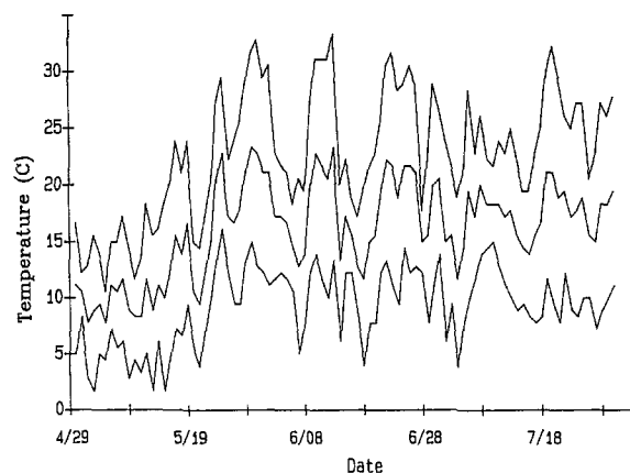
Fig. 1. Occurrence of maximum, mean, and minimum daily temperatures ( ^{\circ}\text{C} ) during the study period. Corvallis, Oreg. 1986.
