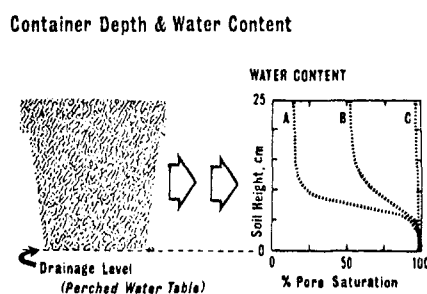
Figure 5. A perched water table forms at the container bottom following irrigation and drainage, and water content decreases with height above the bottom. Line A indicates the water distribution pattern for a very coarse-textured sand; C, a silty clay loam soil; and B a mixture of A and C.
