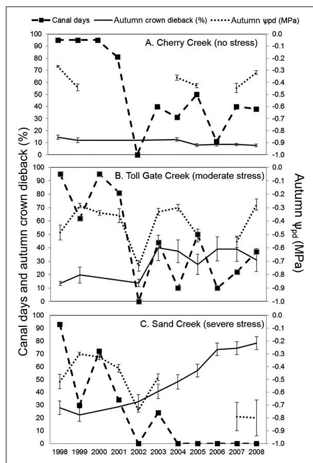
Figure 3. Days of canal flow and yearly means ( \pm one standard error) of percent autumn crown dieback and autumn predawn leaf water potentials ( \psi_{pd} ) (MPa) of plains cottonwood trees on the A) Cherry Creek (n = 8 sites), B) Toll Gate Creek (n = 6 sites), and C) Sand Creek (n = 9 sites) canal sections, High Line Canal, Denver, Colorado (1998–2008). Sites represent various levels of water stress based on number of canal-flow days (no, moderate, and severe stress, respectively). Missing sections indicate no data collected
